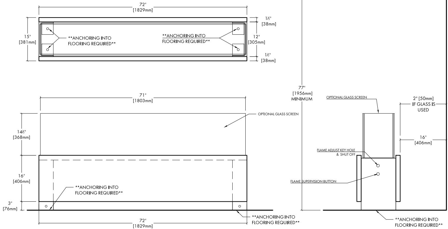
CLEARANCES to ADJACENT MATERIALS
